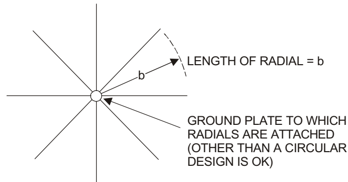
Figure 3-16. Radials.
