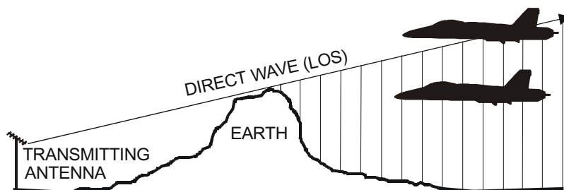
Figure 2-9. UHF LOS.
